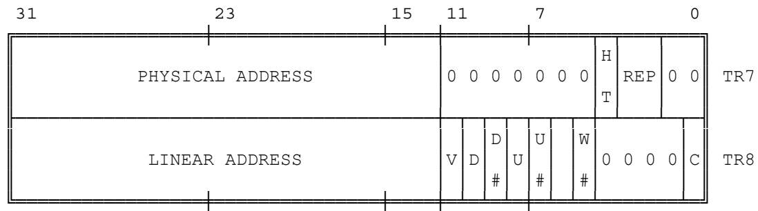
Figure 10-4. Test Registers
