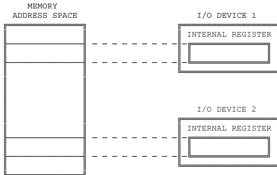
Figure 8-1. Memory-Mapped I/O
