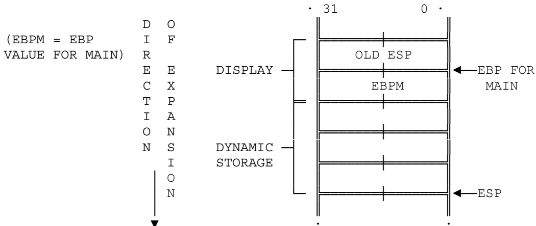
Figure 3-18. Stack Frame for MAIN at Level 1
