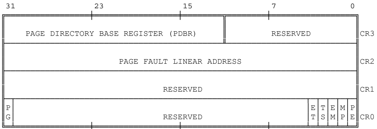
Figure 4-2. Control Registers
