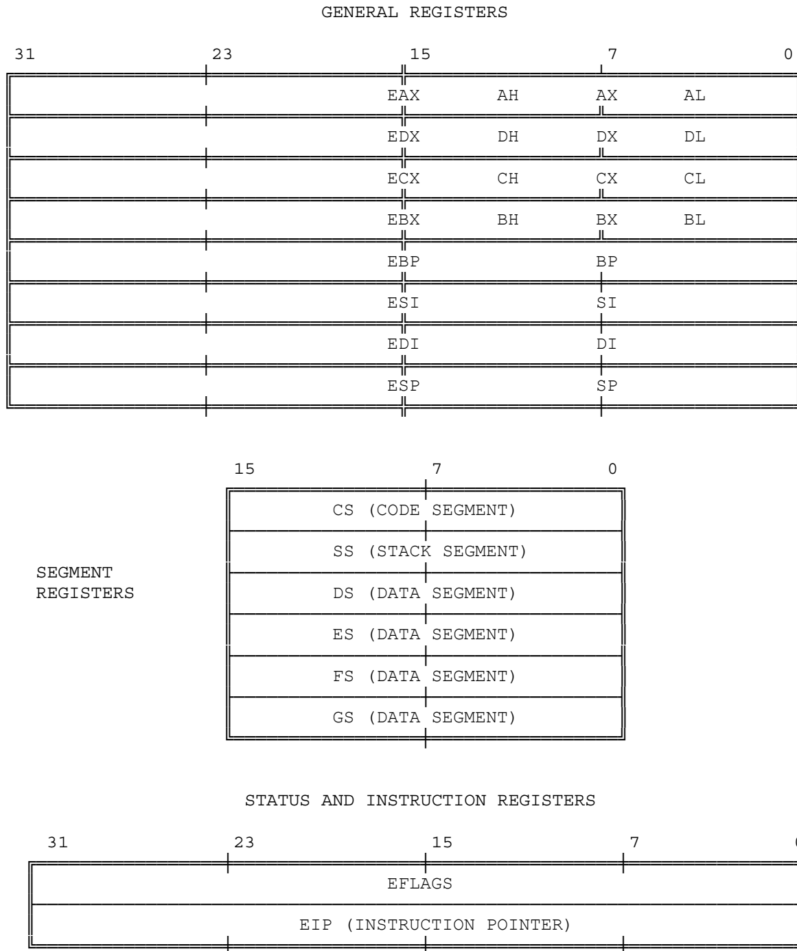
Figure 2-5. 80386 Applications Register Set
